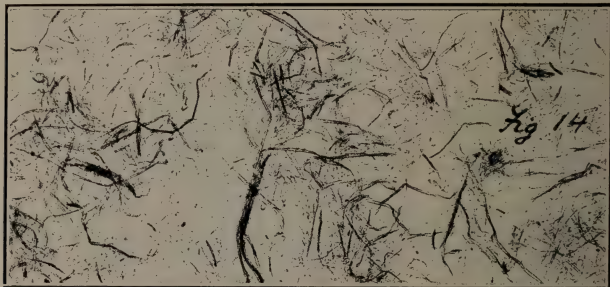
Fig. 14.—Ground-Wood Pulp, All Spruce. (Run No. 46C.)
